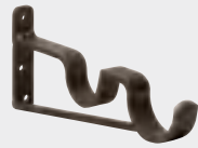
DBL1 custom steel bracket, double please specify: A. front pole size and profile B. back pole size and profile C. rings to be used, if any D. front and back returns (distance from wall to center of cradle) note: returns are contingent upon which poles and rings are chosen 3½"H backplate comes standard, unless otherwise specified
