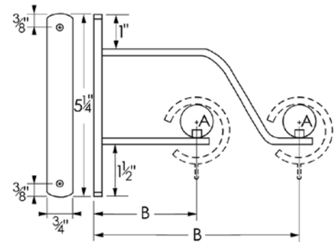
returns will match double cradle brackets used at each end of pole
